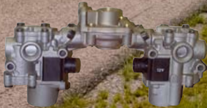
STEER AXLE VALVE PACKAGE
